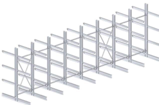
Bundle 8 "9 Upright 54 Arms" – Length 12,00 m
