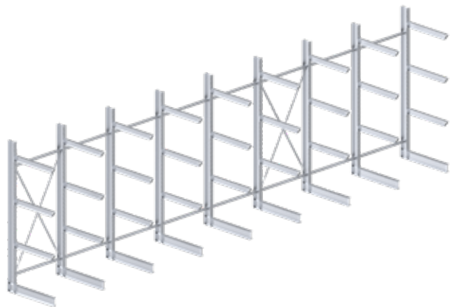
Bundle 4 "9 Upright 27 Arms" – Length 12,00 m
