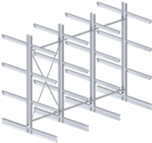
Bundle 5 "4 Upright 24 Arms" – Length 4,50 m
