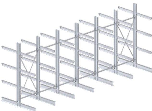
Bundle 7 "7 Upright 42 Arms" – Length 9,00 m
