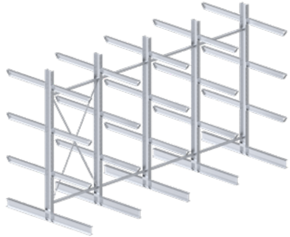
Bundle 6 "5 Upright 30 Arms" – Length 6,00 m
