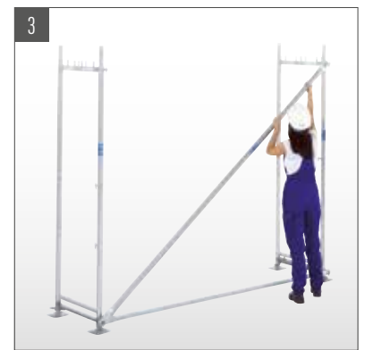
Mount diagonal brace via swivel pins.
